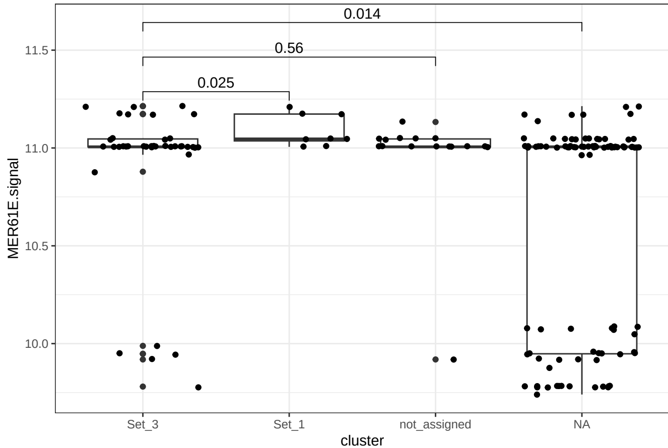
n=156 MER61Es and motif scores for halfsite p53 motif
